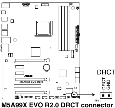
M5A99X EVO R2.0 DRCT connector
