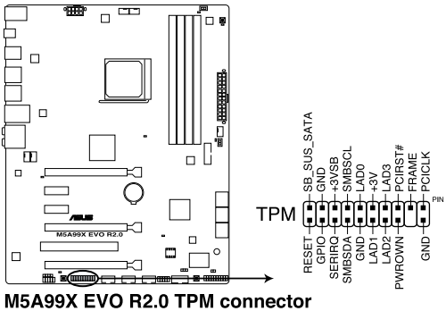
M5A99X EVO R2.0 TPM connector
